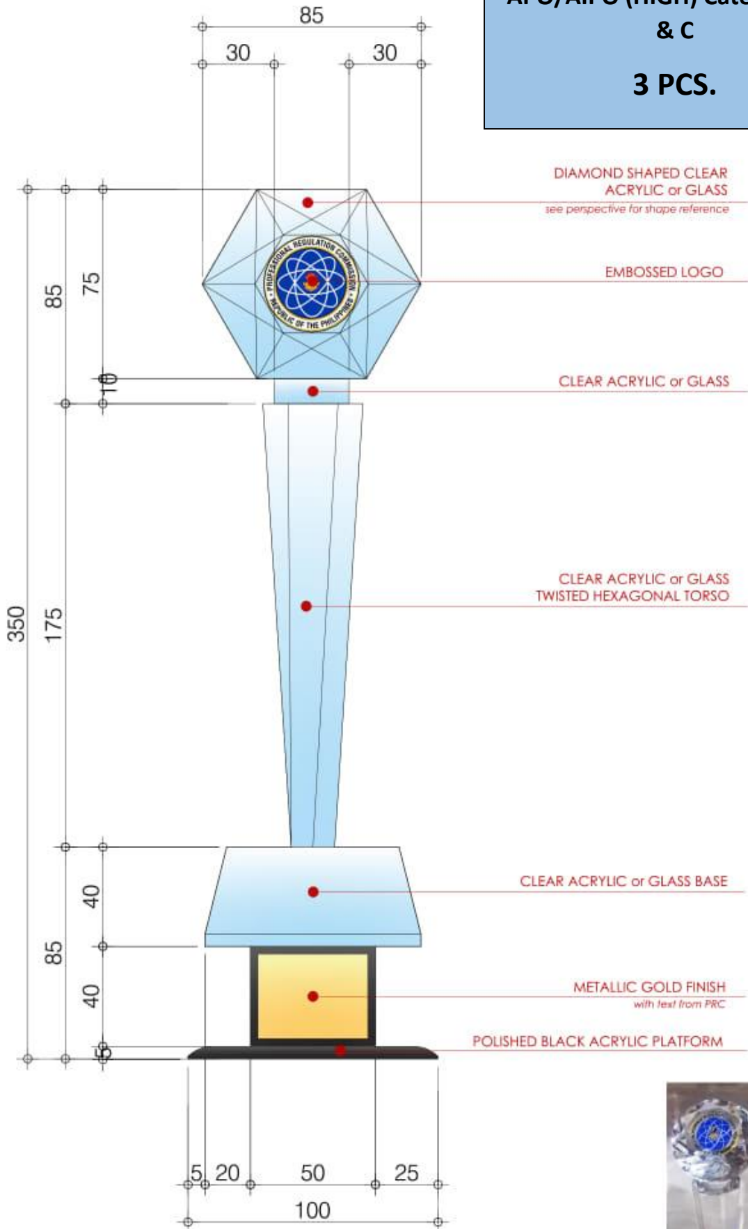
MOST OUTSTANDING IAPOA - LARGE FRONT ELEVATION SCALE 1:2M/TS
