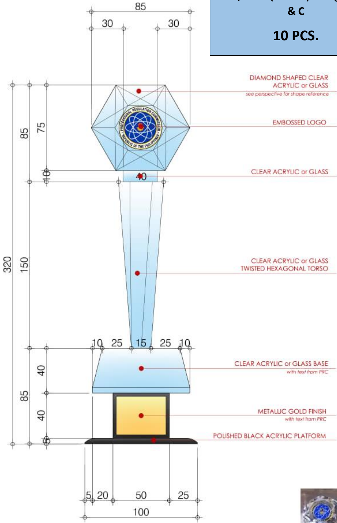
MOST OUTSTANDING IAPOA - SMALL FRONT ELEVATION SCALE 1:2MMS
